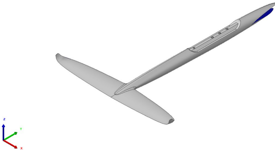
Figure 1 - Definition of the Coordinate System
