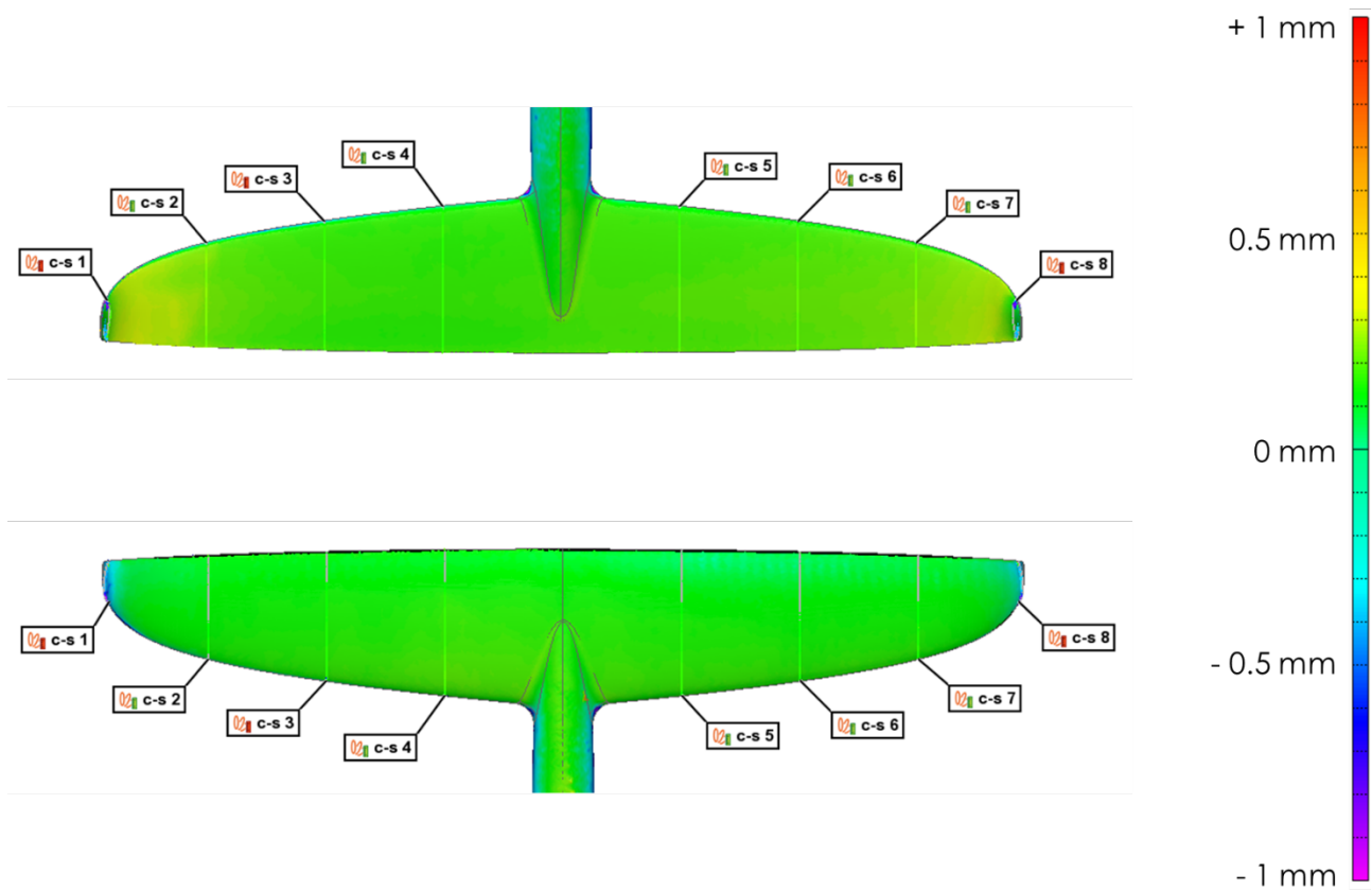
Figure 7 - Colour Map of the Upper (top) and Lower (bottom) surfaces of the Rearwing
