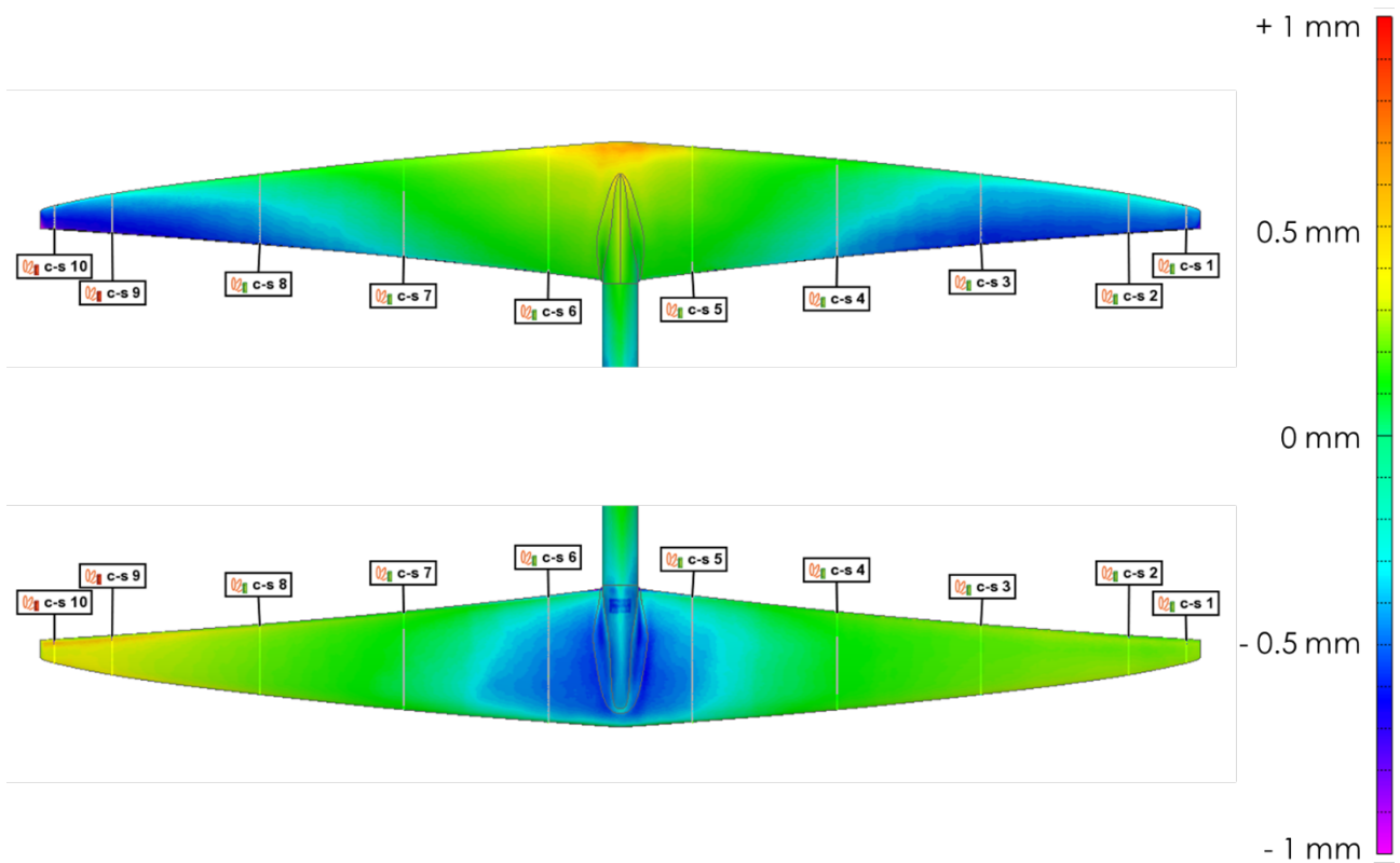
Figure 7 - Colour Map of the Upper (top) and Lower (bottom) surfaces of the Frontwing
