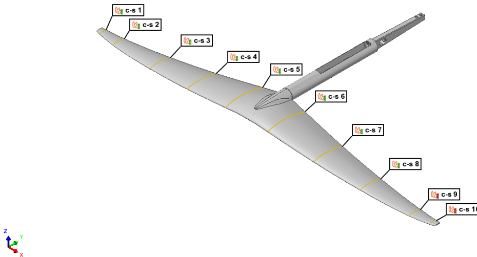
Figure 2 - Definition of Cross Sections
