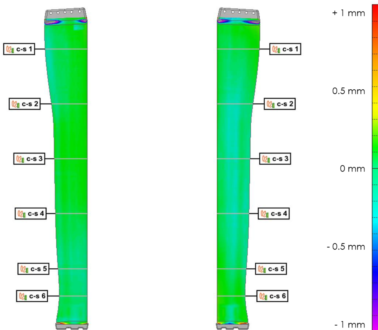
Figure 6 - Colour Map of the Upper (top) and Lower (bottom) surfaces of the Mast
