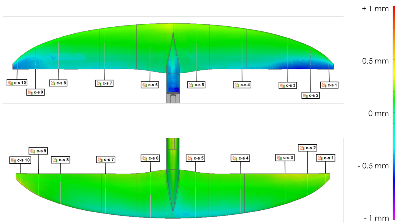
Figure 7 - Colour Map of the Upper (top) and Lower (bottom) surfaces of the Frontwing
