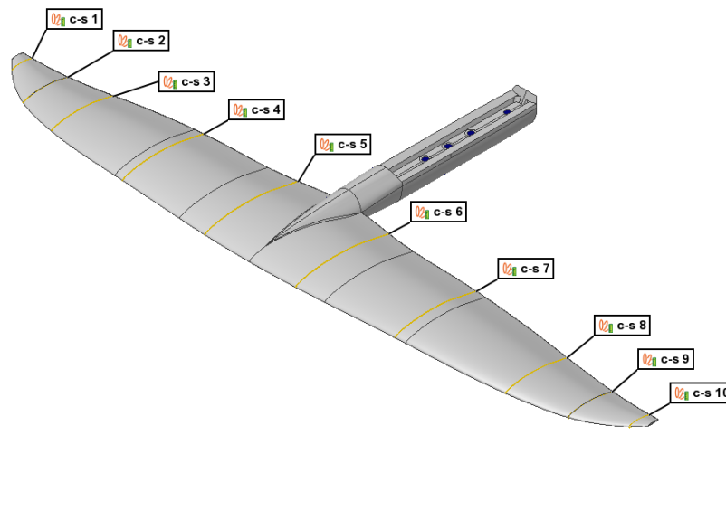
Figure 2 - Definition of Cross Sections
