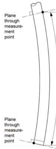
Spar Length Measurements
