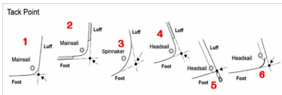
Figure G.2.1.1 Tack point, ERS definition.
