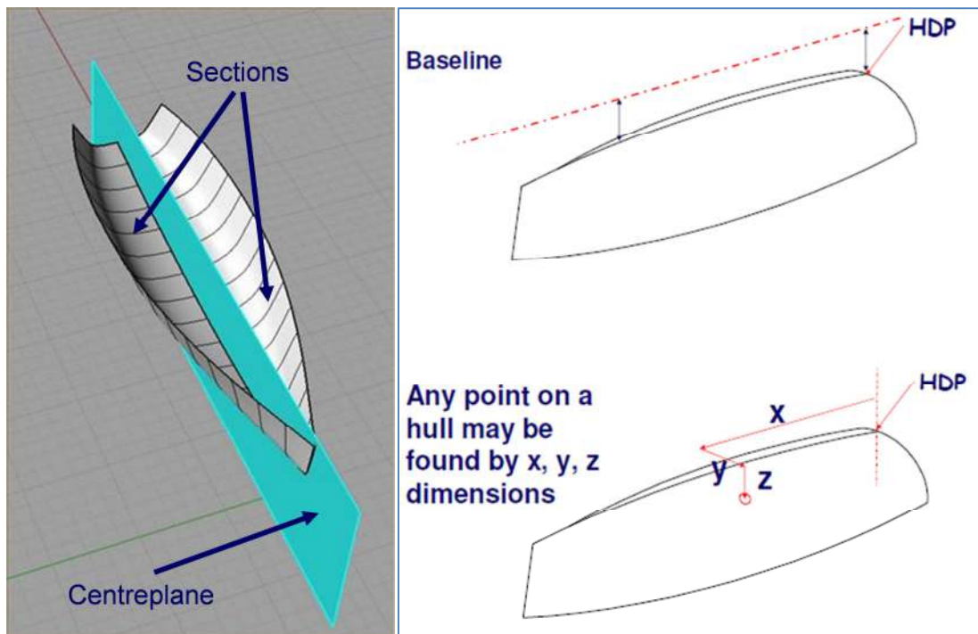
Figure D.2.1 Basic terms
