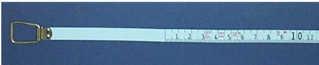
Figure H.4.1 A measuring tape with an offset zero to eliminate end errors.
