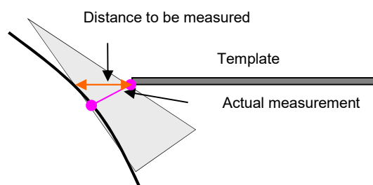
Figure D.5.1.5 Wedge measurement errors
