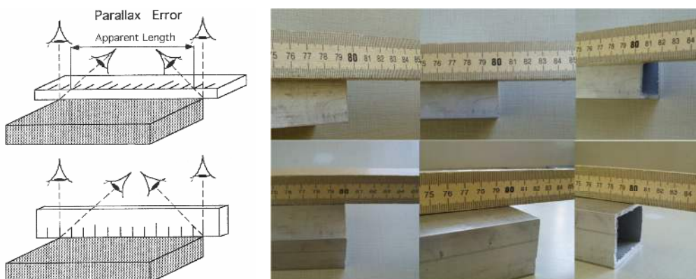
Figure H.4.3 The parallax error when sighting a non-contiguous scale
