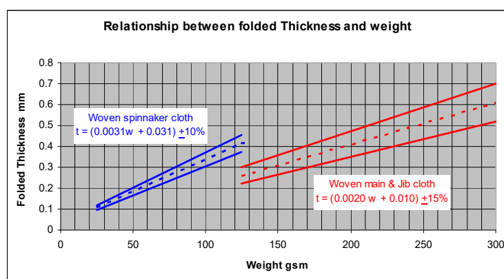
Figure G.1.2.2 Woven ply thickness vs. weight
