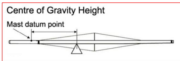
Figure F.5.1.1 Determination of the mast CG by balancing on a knife edge. The knife edge is set at the minimum permitted distance from the datum point and the mast tip must either go down when released or the mast will stay balanced on the knife edge.
