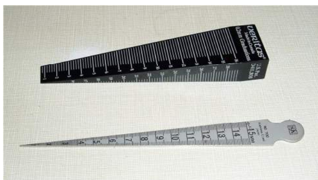
Figure H.4.6 Two types of wedge gauge and the error in gap measurement.
